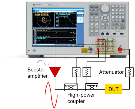
Figure 5. Configuration example using direct receiver access
