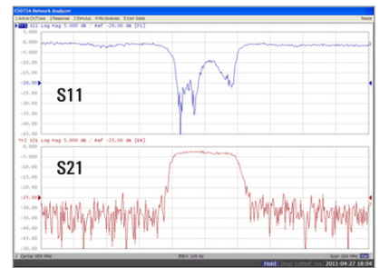
Figure 7. Accurate measurements with low signal input, Upper (power = -55 dBm with external 20 dB attenuator), Lower (power = -75 dBm with built-in attenuator)
