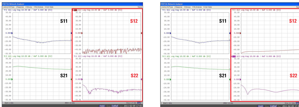
Coupled power (Port 1 = Port 2 = -40 dBm)
